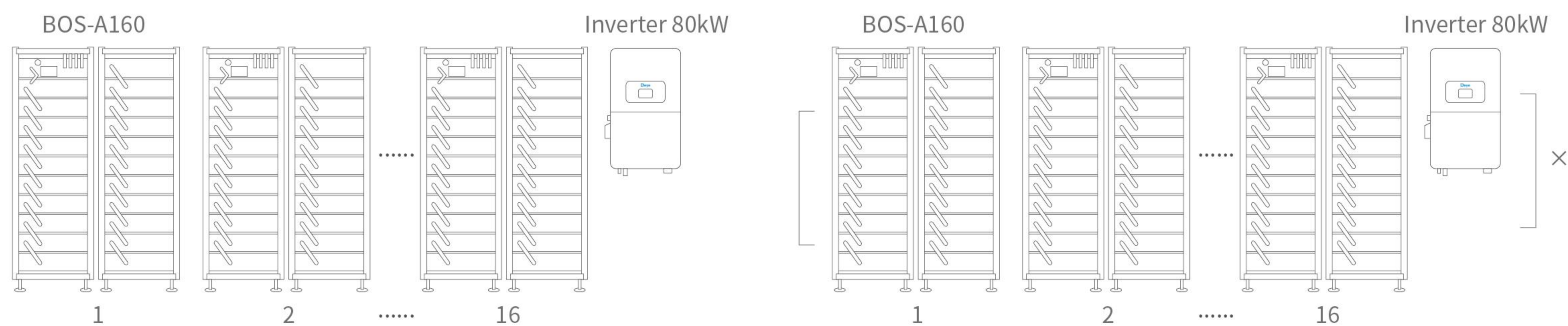
Maximum support for 16 clusters of batteries in parallel Maximum support for 10 inverters in AC parallel operation
