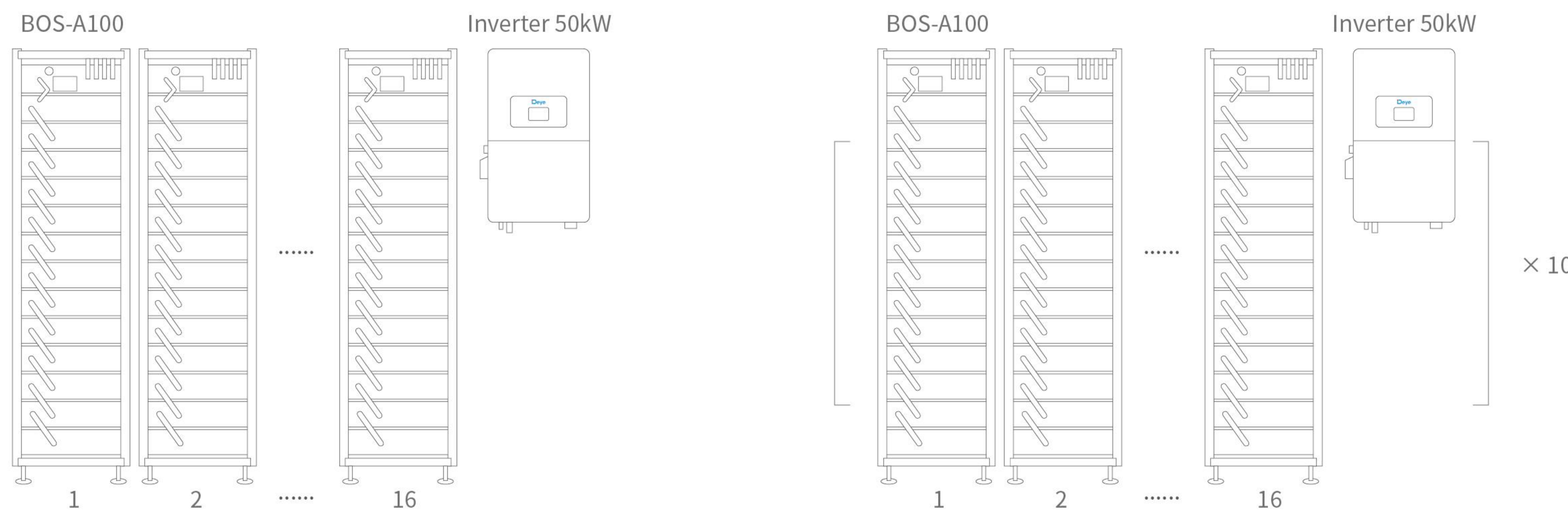
Maximum support for 16 racks of batteries in parallel Maximum support for 10 inverters in AC parallel operation
