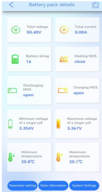
Figure 8: Battery pack details
